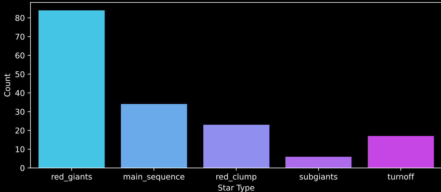
APOGEE DR17 Field: [191+22_MGA] Count plot of Star Type
