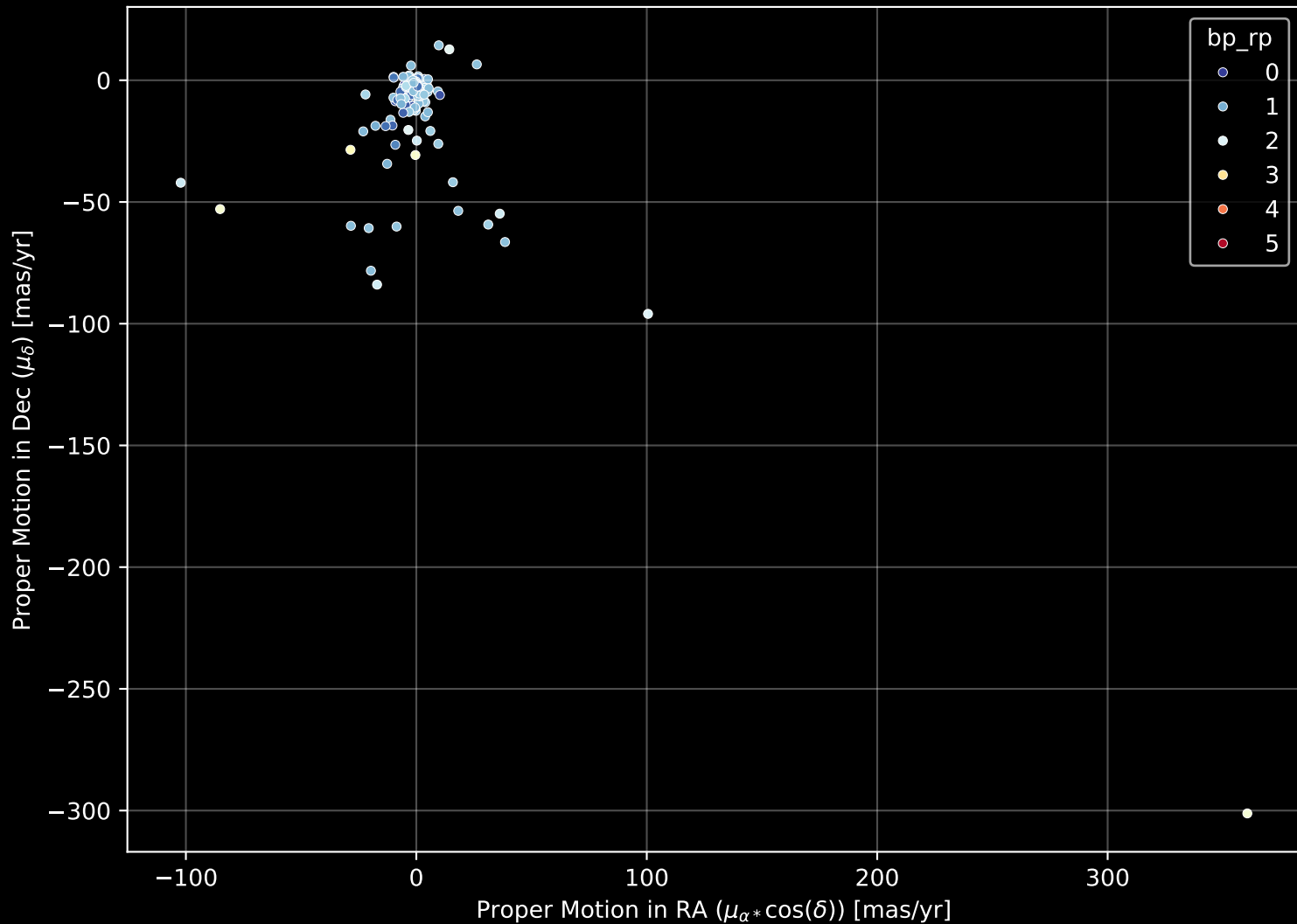
APOGEE DR17 Field: [191+22_MGA] Proper Motion Diagram (n= 164)
