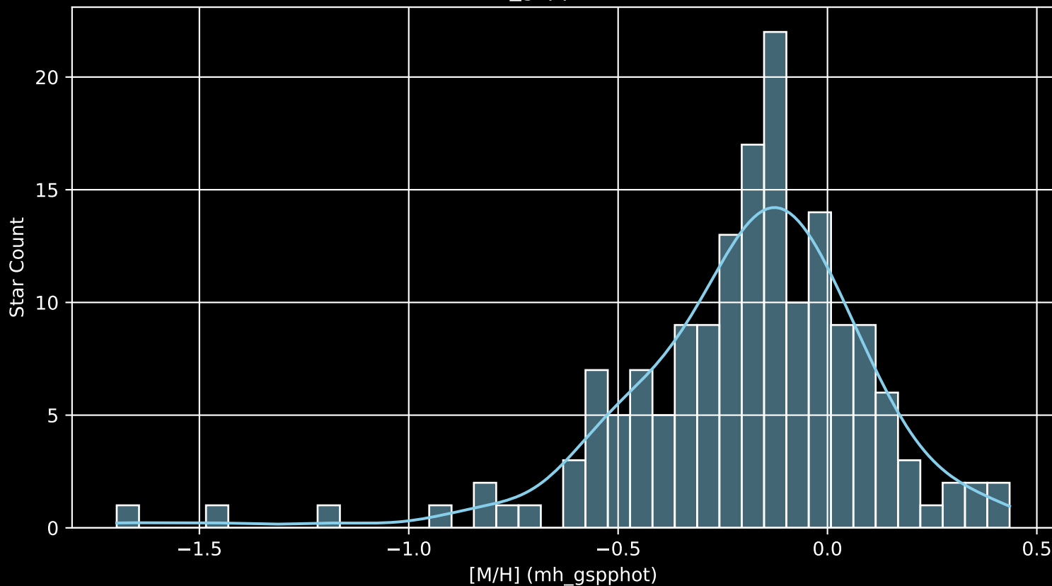
APOGEE DR17 Field: [191+22_MGA [M/H] (mh_gspphot) (n= 163)
