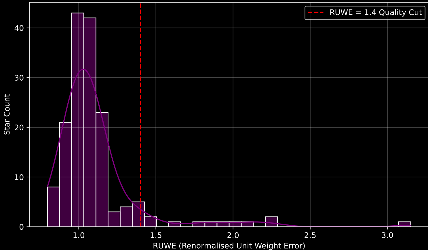
GAPOGEE DR17 Field [191+22_MGA] RUWE Distribution (n= 160)
