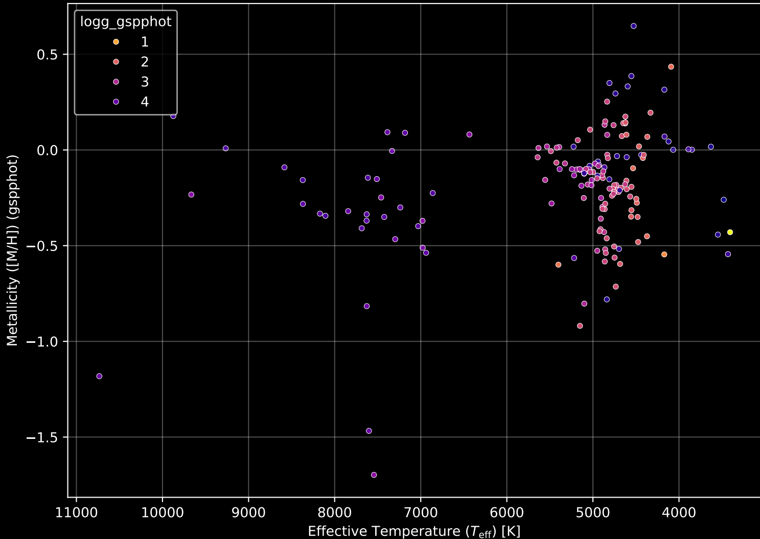
APOGEE DR17 Field: [191+22_MGA] Stellar Population Parameters (n= 164)
