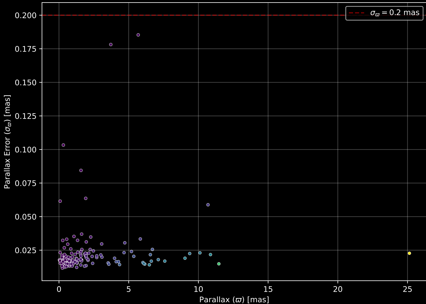
APOGEE DR17 Field: [191+22_MGA] Parallax Quality (n= 164)
